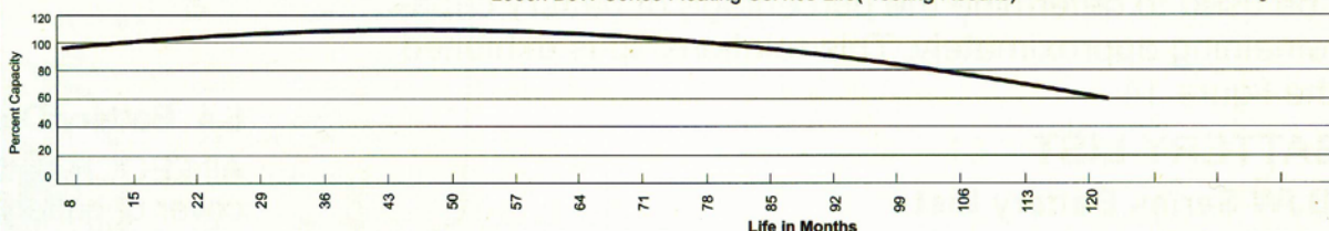
Leoch DJW Series Floating Service Life( Testing Results)
