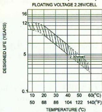
Figure 9. Effect Of Temperature On Long Term Float Life (DJW series)
