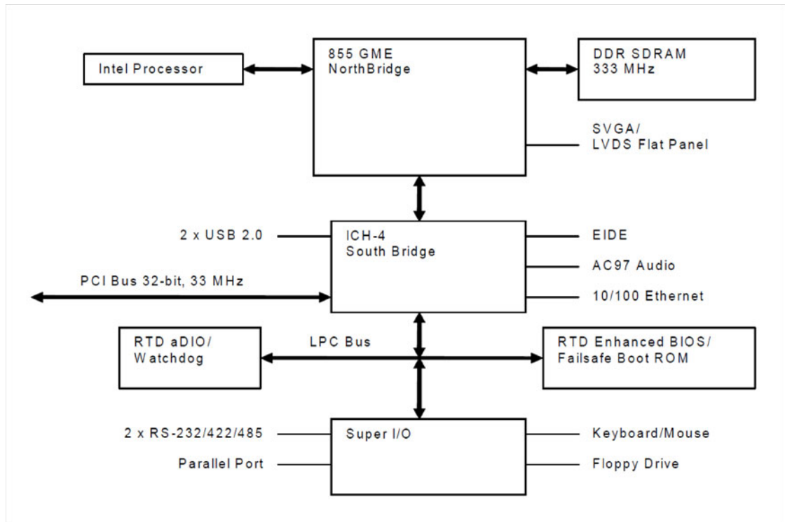
Figure 2 CMX158886 cpuModule Simplified Block Diagram
